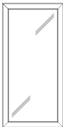
Fully Glazed WxH 890mm x 1820mm
